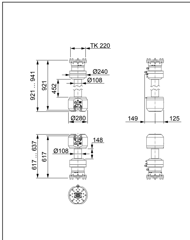
Hydraulic grip 250 kN for temperature chambers, dimensions
